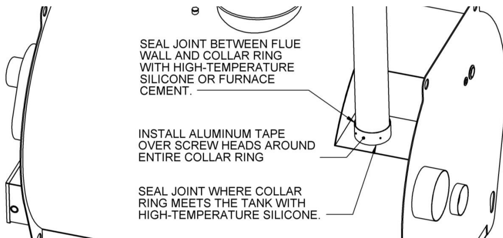
VERTICAL FLUE - FIGURE 3:
