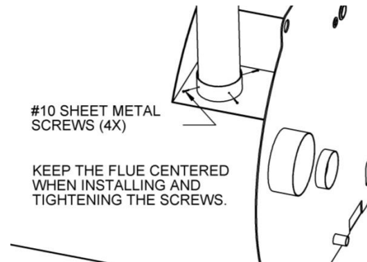
VERTICAL FLUE - FIGURE 2:
