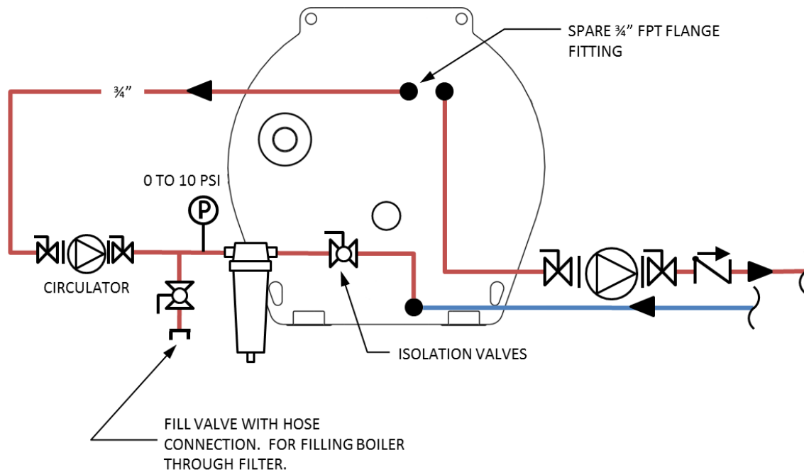
Figure 1: HWR to Spare Flange
