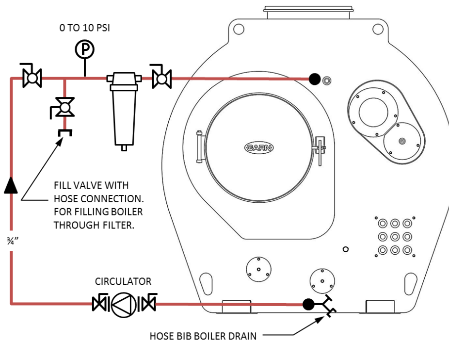
Figure 2: Boiler Drain to Spare Flange
